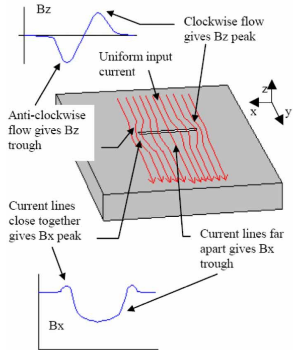
Fig. 11 Definition of field directions and co-ordinate system used in ACFM (taken from reference [74])
