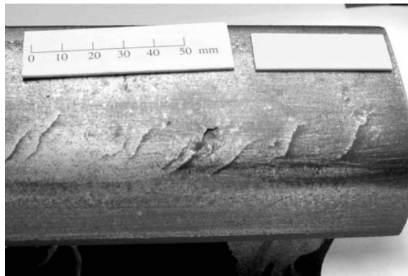
Fig. 1 RCF damage on a rail section
