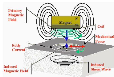
Fig. 12 EMAT principle (taken from reference [77])
